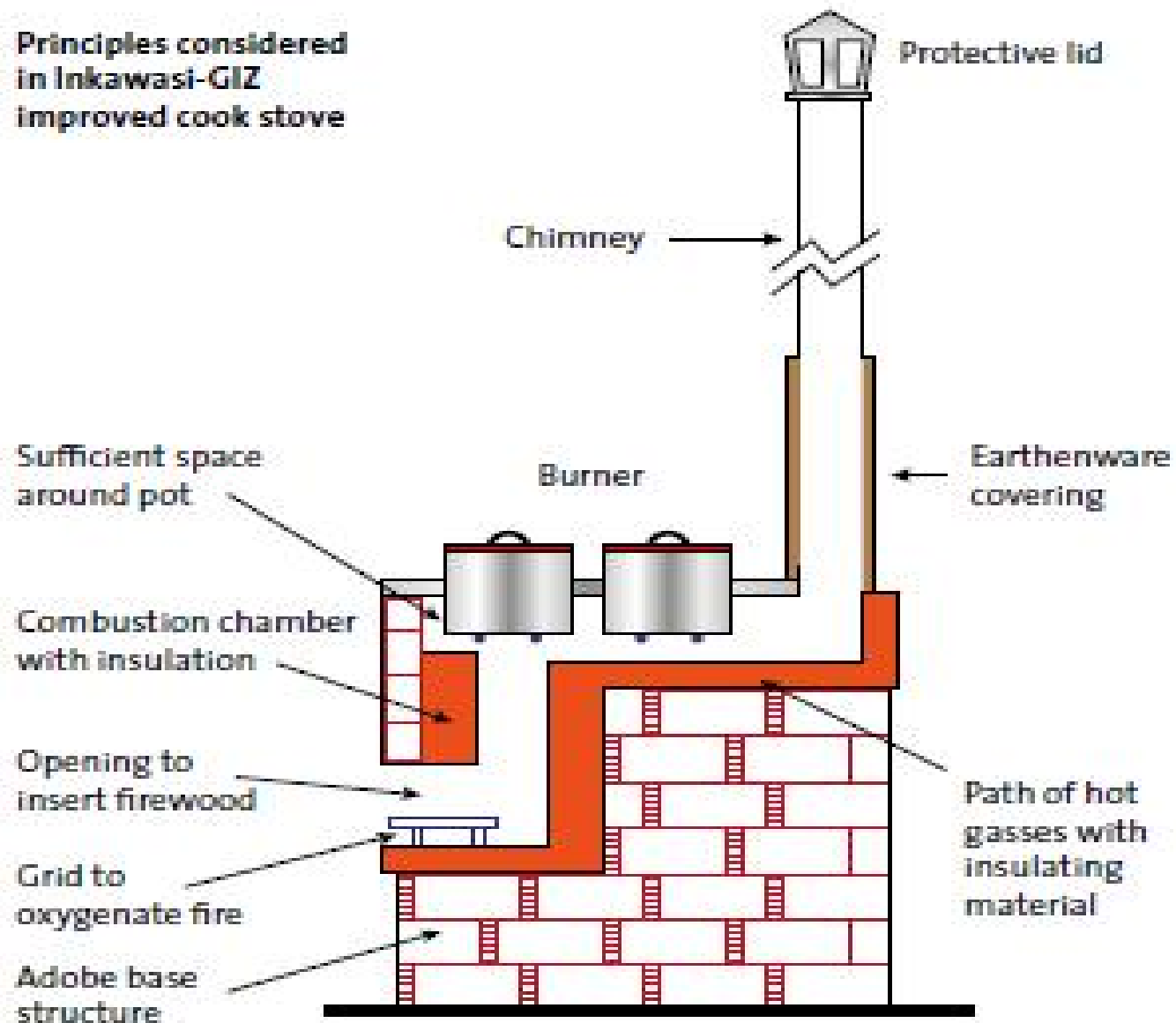
Figure 9. General diagram of improved Inkawasi cookstove (13)
