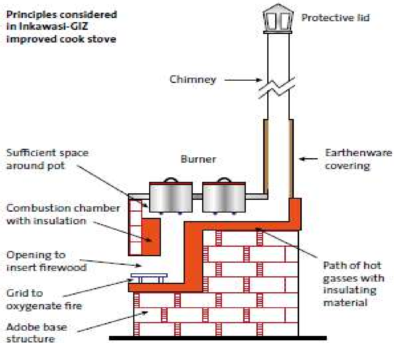
Figure 9. General diagram of improved Inkawasi cookstove (13)
