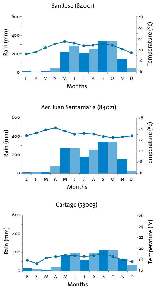
Figure 2. Climatology of three seasons in three major cities in Valle Central in Costa Rica
